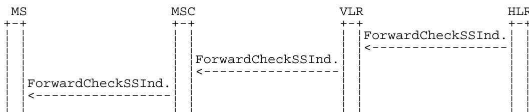
Figure 6.8: ForwardCheckSSIndication
