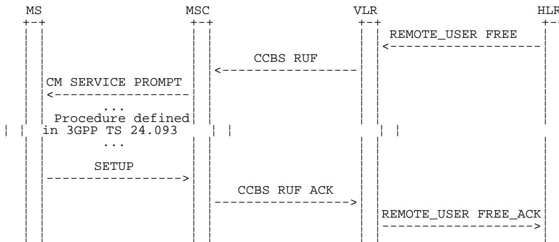
Figure 6.9: Signalling for CCBS Recall
