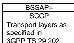
Figure 4.1: Protocol stack for the transportation of BSSAP+
