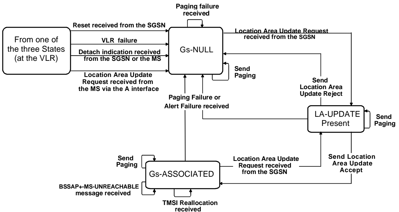
Figure 4.1/GSM 29.018: State diagram at the VLR
