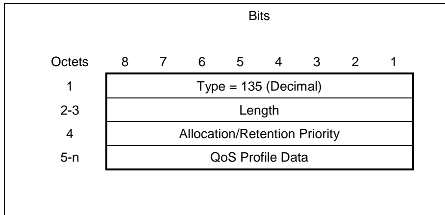
Figure 48: Quality of Service (QoS) Profile Information Element
