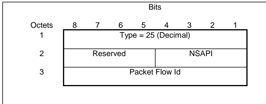
Figure 30: Packet Flow Id Information Element
