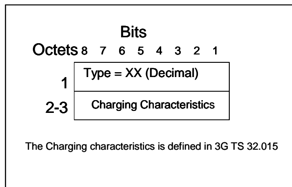
Figure 31: Charging Characteristics Information Element
