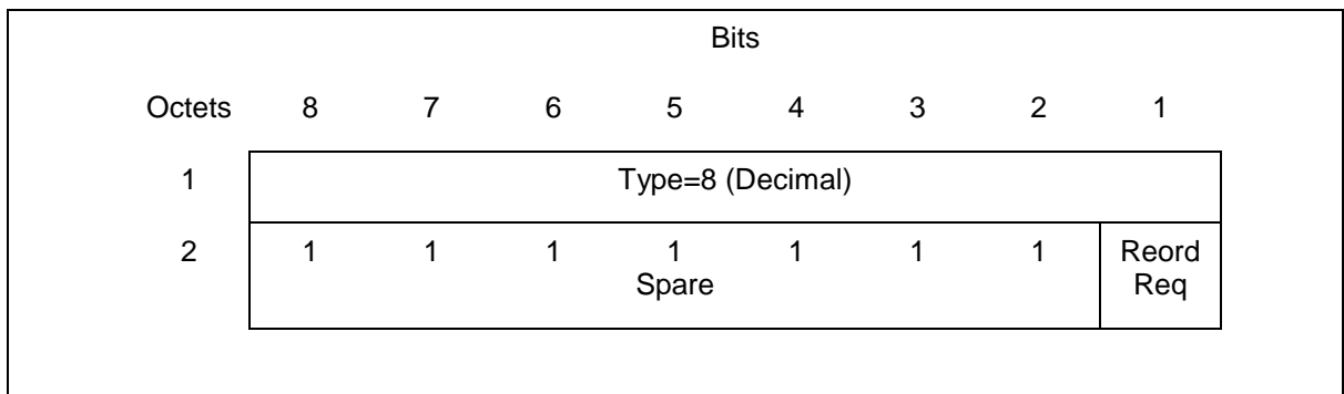
Figure 14: Reordering Required Information Element
