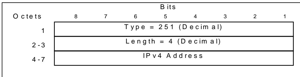
Figure 58: Charging Gateway Address Information Element
