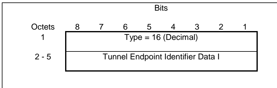
Figure 21: Tunnel Endpoint Identifier Data Information Element
