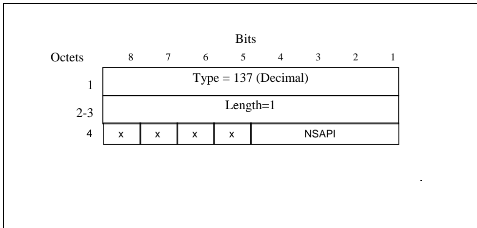
Figure 54: RAB Setup Information information element for release of resources
