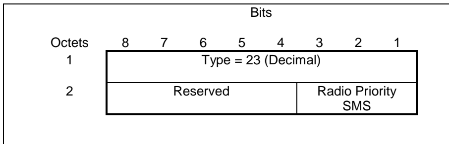
Figure 28: Radio Priority SMS Information Element
