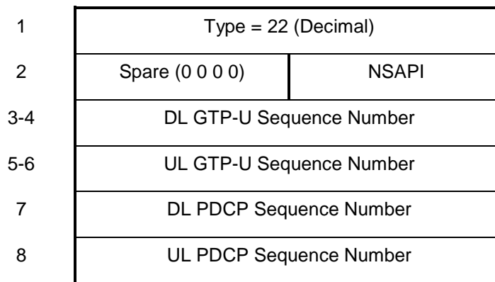
Figure 27: RAB Context Information Element
