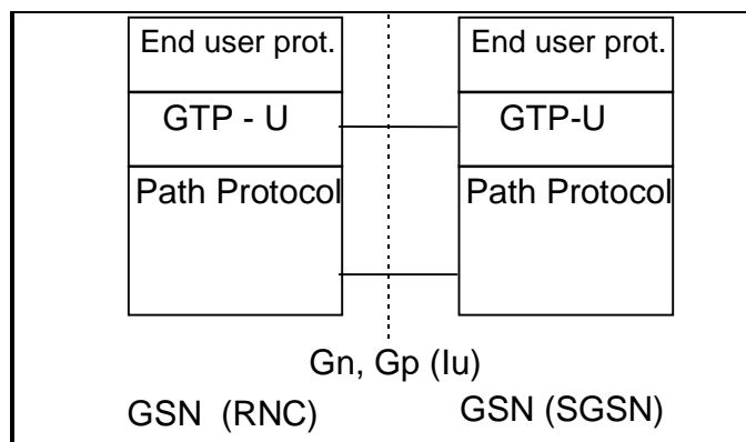
Figure 63: GTP-U - Protocol Stack (GTP-U over the Iu in brackets)
