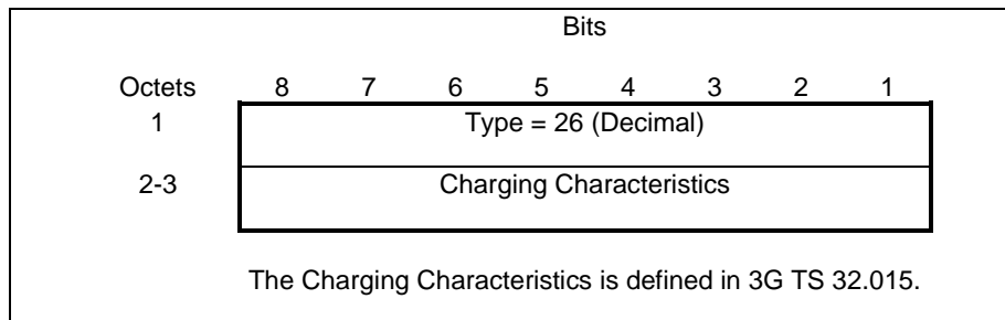
Figure 31: Charging Characteristics Information Element
