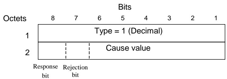
Figure 9: Cause information element
