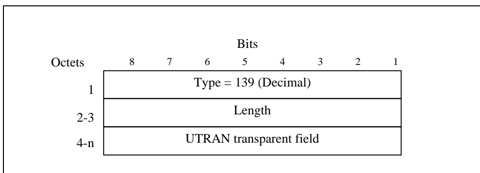
Figure 52: UTRAN Transparent Container Information Element
