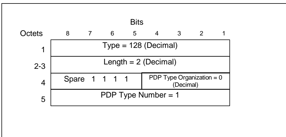
Figure 38: End User Address Information Element for PPP
