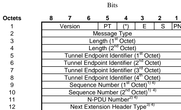
Figure 2: Outline of the GTP Header
