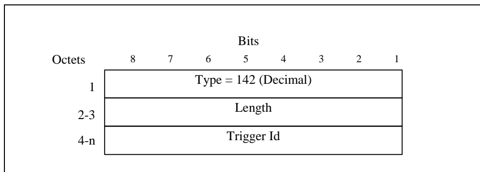
Figure 56: Trigger Id Information Element
