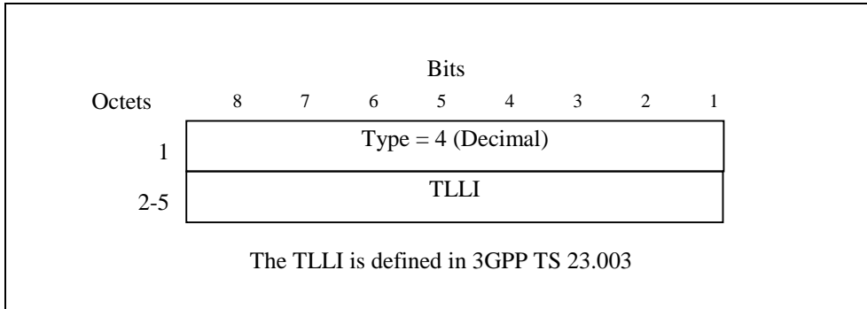
Figure 12: TLLI Information Element
