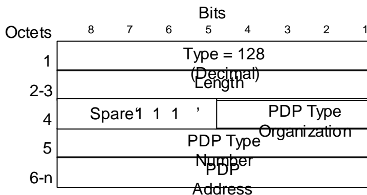
Figure 35: End User Address Information Element
