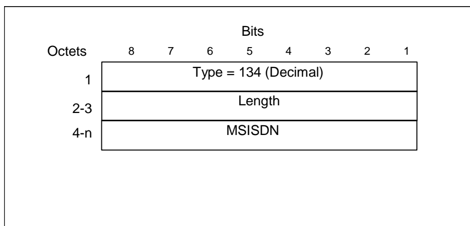
Figure 47: MSISDN Information Element
