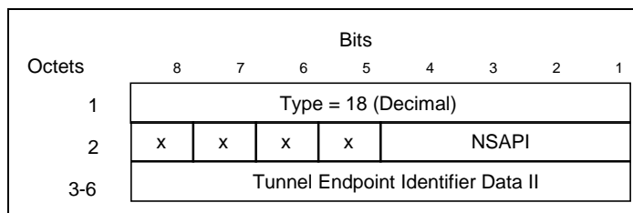
Figure 23: Tunnel Endpoint Identifier Data II Information Element
