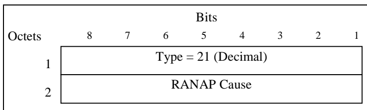
Figure 26: RANAP Cause Information Element
