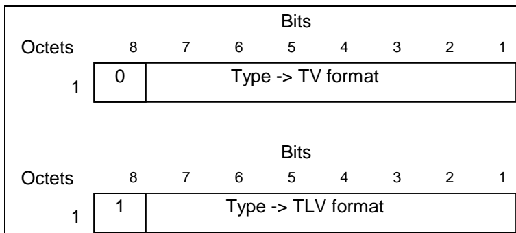
Figure 8a: Type field for TV and TLV format
