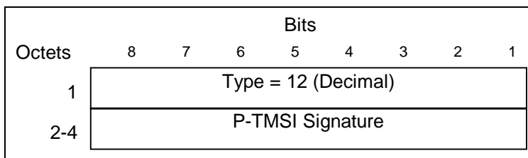
Figure 17: P-TMSI Signature Information Element
