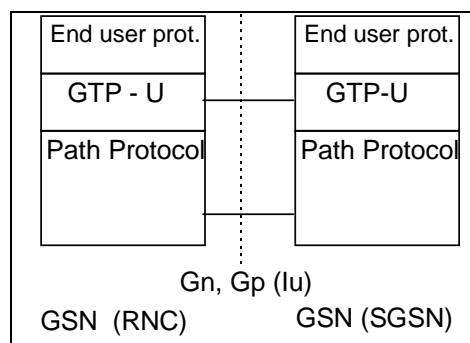
Figure 63: GTP-U - Protocol Stack (GTP-U over the lu in brackets)
