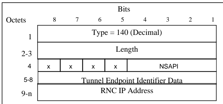
Figure 53: RAB Setup Information IE for data forwarding
