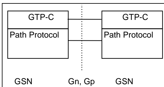
Figure 60: Signalling Plane - Protocol Stack
