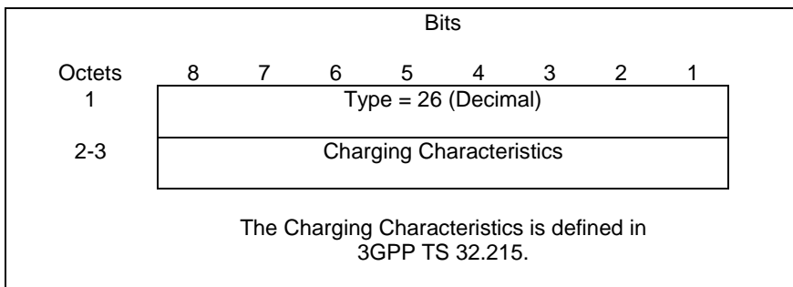
Figure 31: Charging Characteristics Information Element
