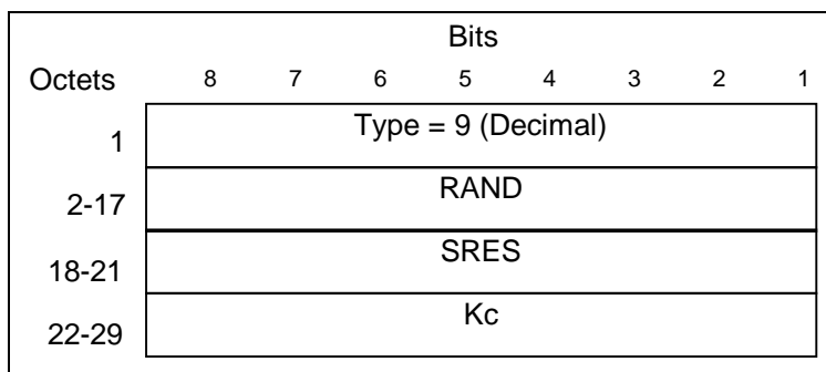
Figure 15: Authentication Triplet Information Element
