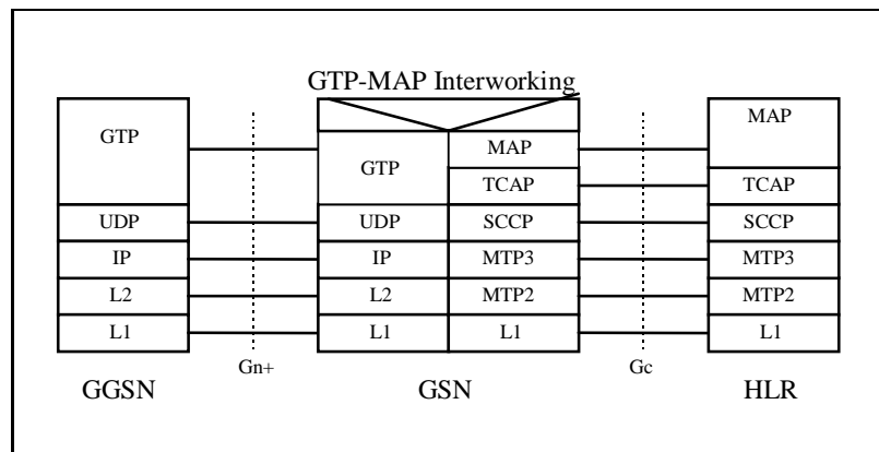
Figure 7a: GGSN - HLR Signalling via a GTP-MAP Protocol-Converter in a GSN
