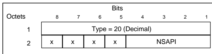
Figure 25: NSAPI Information Element
