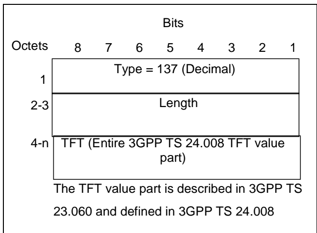
Figure 50: Traffic Flow Template Information Element
