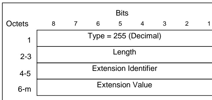
Figure 59: Private Extension Information Element
