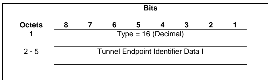
Figure 21: Tunnel Endpoint Identifier Data I Information Element
