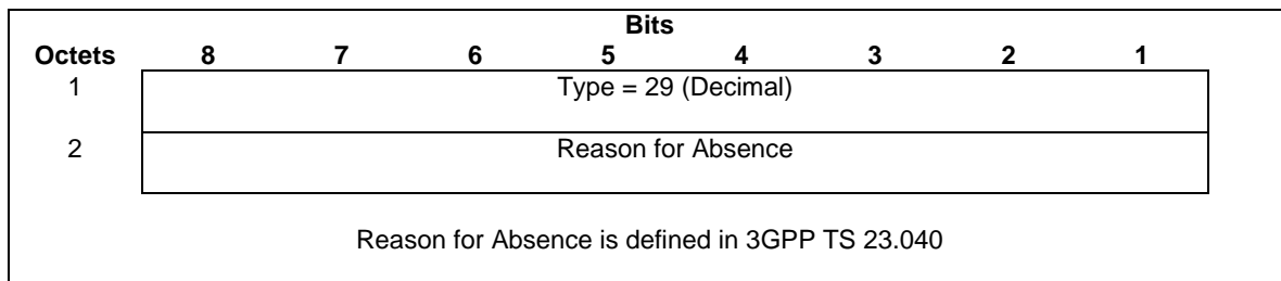
Figure 33A: MS Not Reachable Reason Information Element
