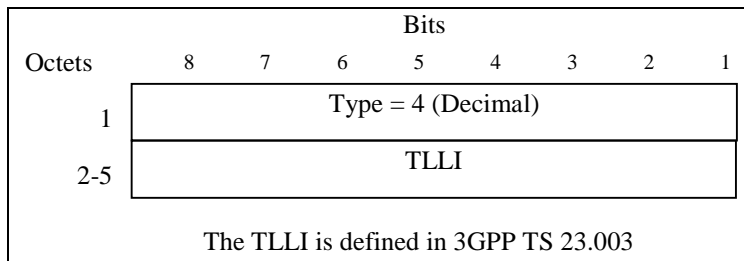
Figure 12: TLLI Information Element
