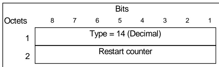
Figure 19: Restart Counter Information Element
