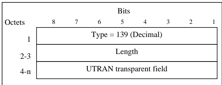
Figure 52: UTRAN Transparent Container Information Element
