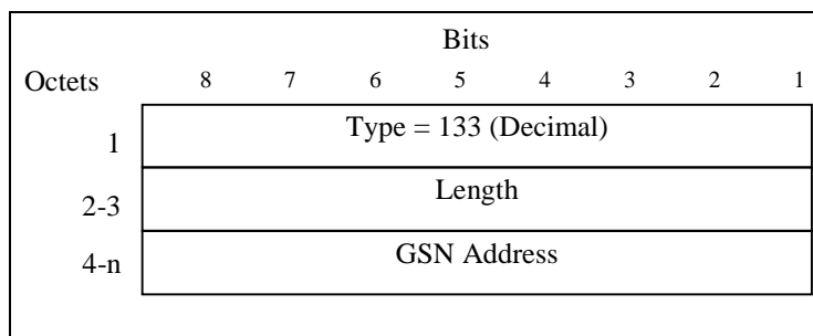
Figure 46: GSN Address Information Element
