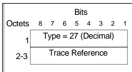
Figure 32: Trace Reference Information Element
