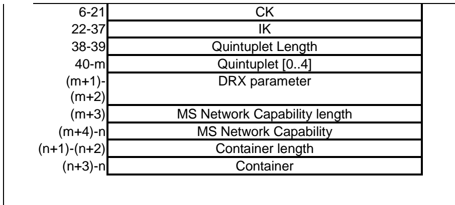
Figure 42A: MM Context Information Element with Used Cipher value, UMTS Keys and Quintuplets
