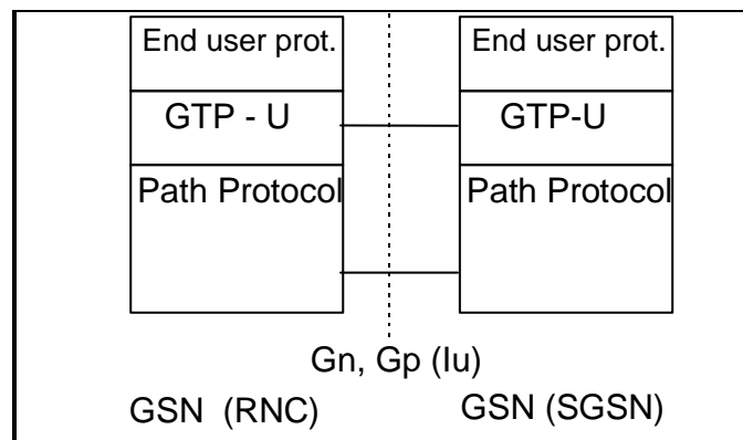
Figure 65: GTP-U - Protocol Stack (GTP-U over the Iu in brackets)
