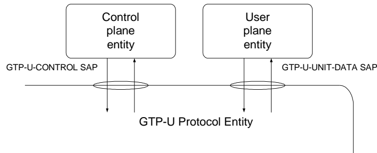
Figure 64: The GTP-U-Control SAP and GTP-U-DATA SAP
