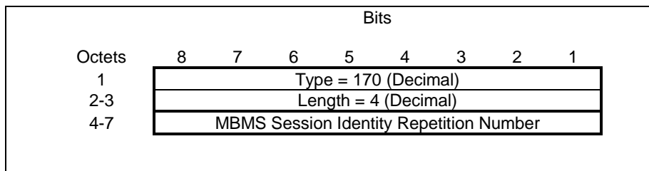
Figure 7.7.69.1: MBMS Session Identity Repetition Number Information Element
