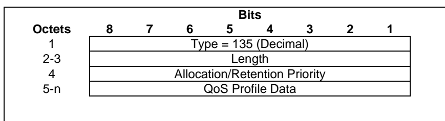
Figure 48: Quality of Service (QoS) Profile Information Element
