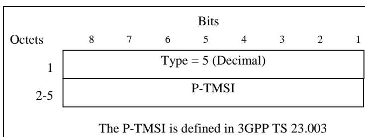
Figure 13: The Packet TMSI Information Element
