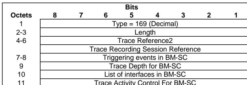
Figure 7.7.68.1: Additional MBMS Trace Info Information Element
