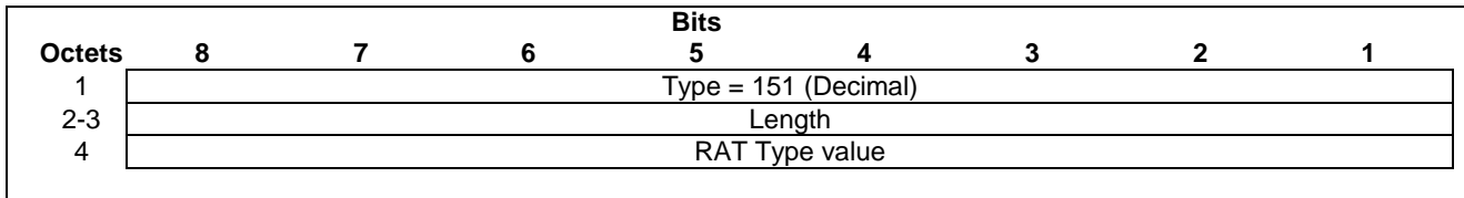
Figure 7.7.50.1: RAT Type Information Element
