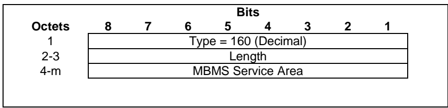
Figure 7.7.60.1: MBMS Service Area Information Element
