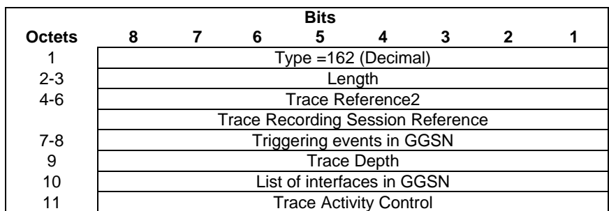
Figure 7.7.62.1: Additional Trace Info Information Element
