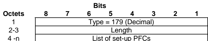
Figure 7.7.78.1: List of set-up PFCs Information Element
