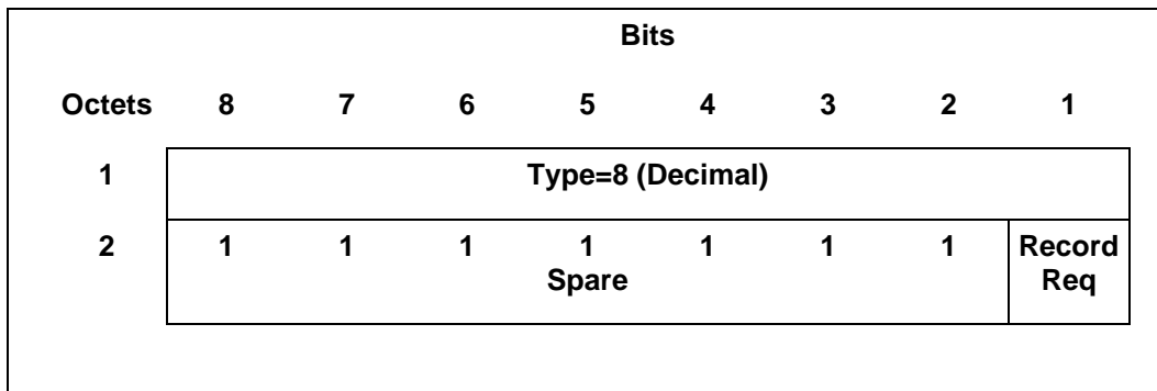
Figure 14: Reordering Required Information Element
