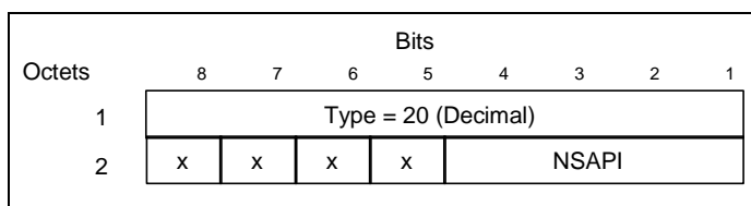
Figure 25: NSAPI Information Element
