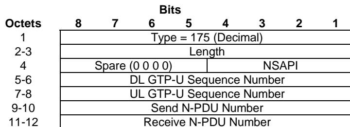
Figure 7.7.74.1: PDU Numbers Information Element
