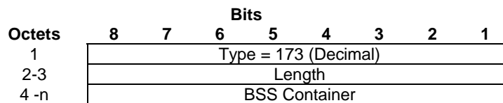
Figure 7.7.72.1: BSS Container Information Element
