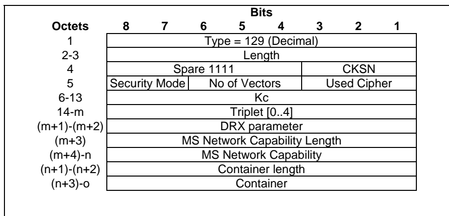
Figure 40: MM Context Information Element with GSM Key and Triplets
