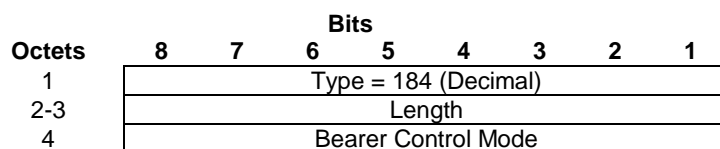
Figure 7.7.83.1: Bearer Control Mode Information Element
