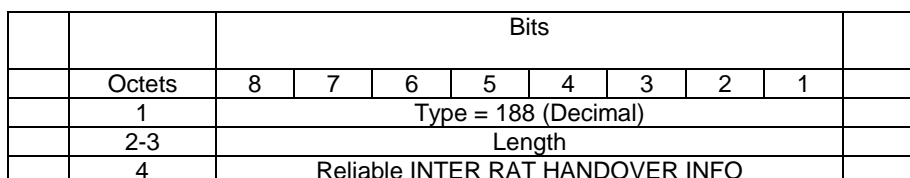
Figure 7.7.84.1: Reliable INTER RAT HANDOVER INFO
