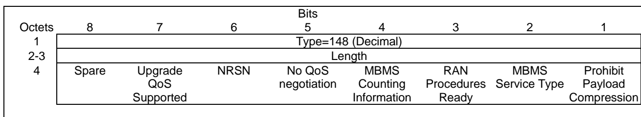
Figure 62a: Common Flags Information Element
