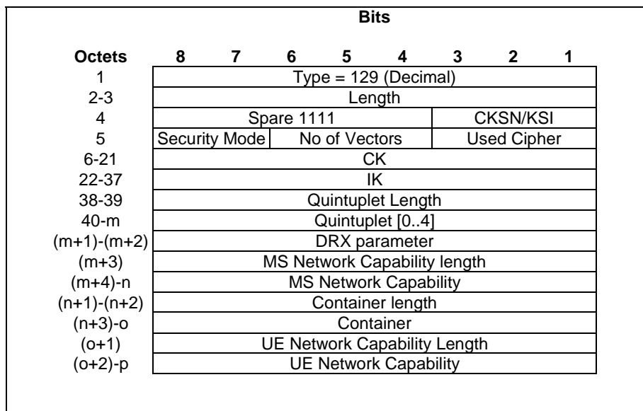
Figure 42A: MM Context Information Element with Used Cipher value, UMTS Keys and Quintuplets
