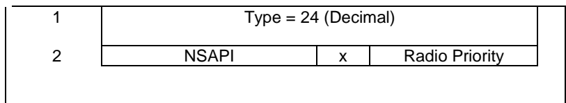
Figure 29: Radio Priority Information Element
