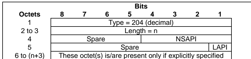
Figure 7.7.104-1: Signalling Priority Indication with NSAPI
