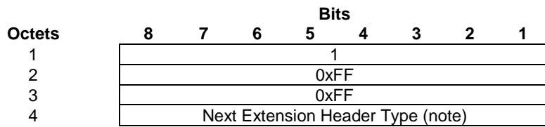
Figure 8A: MBMS support indication Extension Header
