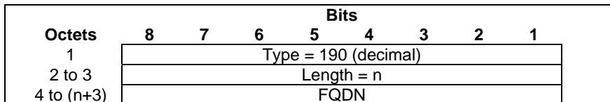
Figure 7.7.x.1: Fully Qualified Domain Name (FQDN)
