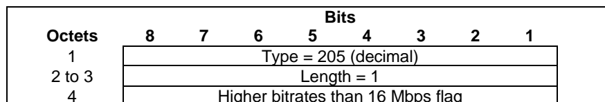
Figure 7.7.105-1: Higher bitrates than 16 Mbps flag
