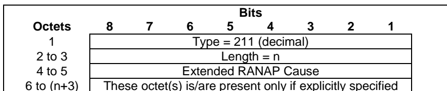
Figure 7.7.111.1: Extended RANAP Cause Information Element
