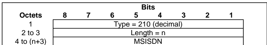
Figure 7.7.110-1: C-MSISDN
