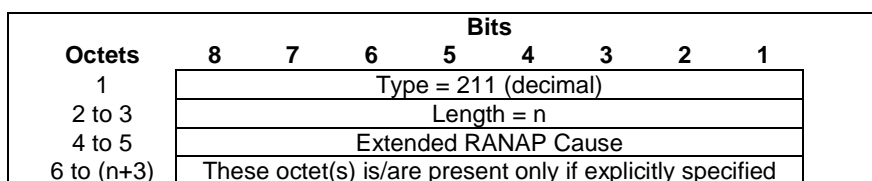
Figure 7.7.111.1: Extended RANAP Cause Information Element
