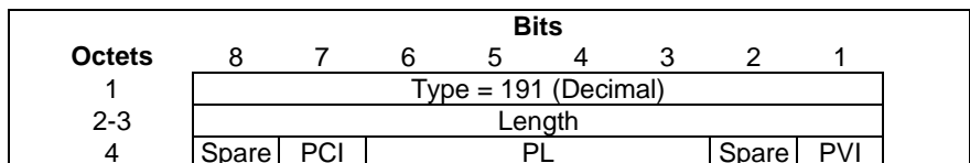
Figure 7.7.91.1: Evolved Allocation/Retention Priority Information Element
