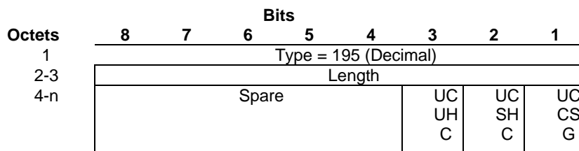
Figure 7.7.95.1: CSG Information Reporting Action
