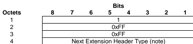
Figure 6.1.5/1: MS Info Change Reporting support indication Extension Header
