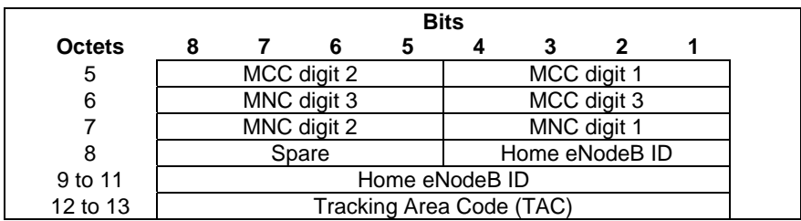
Figure 7.7.112-3: eNodeB ID for Type Home eNodeB
