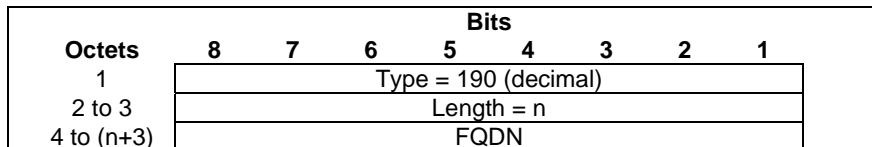
Figure 7.7.90.1: Fully Qualified Domain Name (FQDN)
