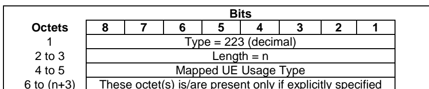
Figure 7.7.123-1: Mapped UE Usage Type
