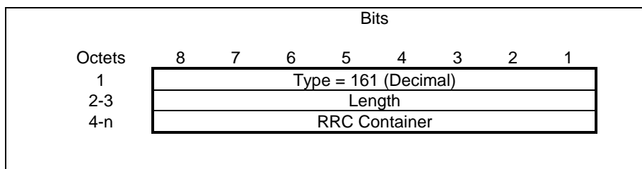
Figure 7.7.61.1: Source RNC PDCCP context info Information Element
