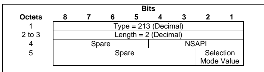
Figure 7.7.113-1: Selection Mode with NSAPI Information Element
