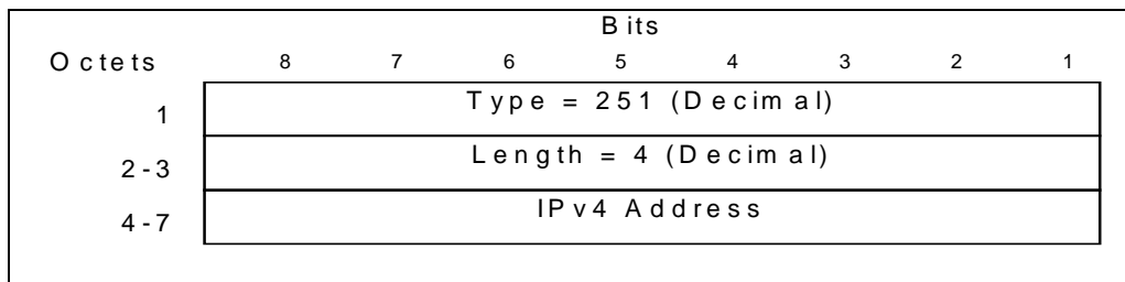
Figure 59a: Ipv4 Charging Gateway Address Information Element
