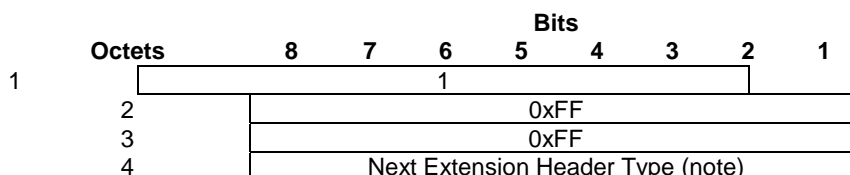
Figure 6.1.5/1: MS Info Change Reporting support indication Extension Header
