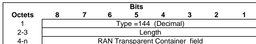
Figure 58: RAN Transparent Container Information Element
