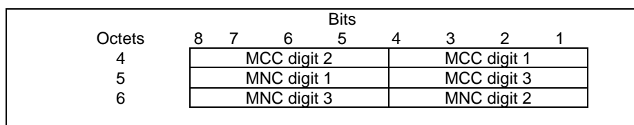
Figure 7.7.64.2: Selected PLMN ID Parameter with 3-digit MNC
