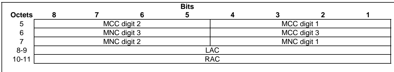
Figure 7.7.51.4: Geographic Location field for RAI
