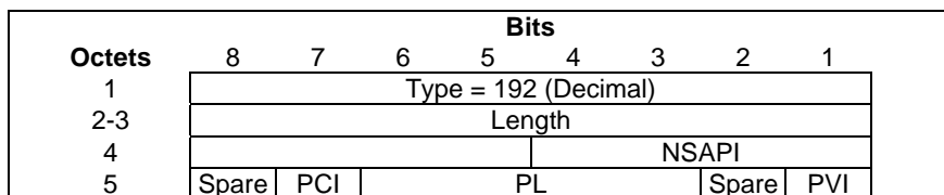
Figure 7.7.92.1: Evolved Allocation/Retention Priority II Information Element
