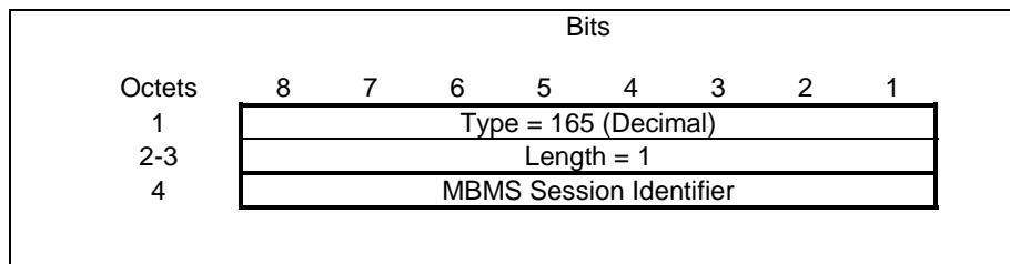
Figure 7.7.65.1: MBMS Session Identifier
