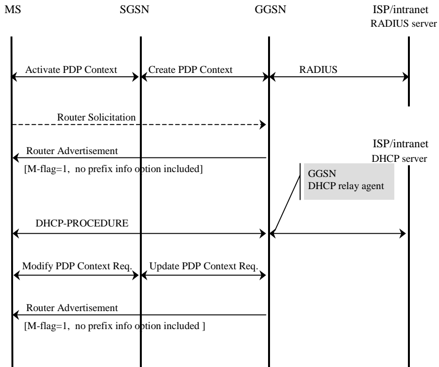
Figure 11bc: IPv6 Stateful Address Autoconfiguration
