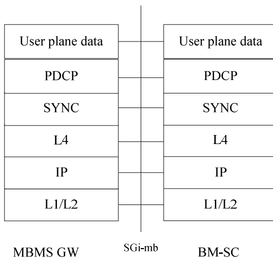
Figure 16k: The user plane protocol stacks of MBMS GW for interworking with BM-SC
