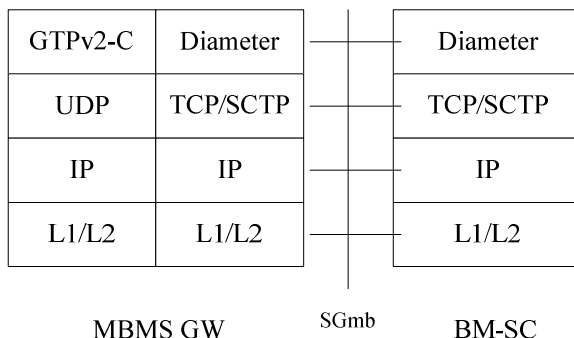
Figure 16j: The control plane protocol stacks of MBMS GW for interworking with BM-SC
