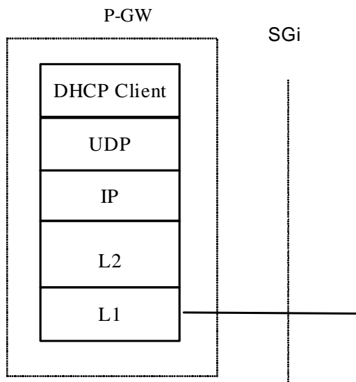
Figure 16g: The protocol stacks for the SGi IP reference point for DHCP
