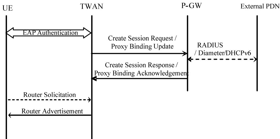
Figure 11be: IPv6 Stateless Address Autoconfiguration for GTP/PMIP-based S2a
