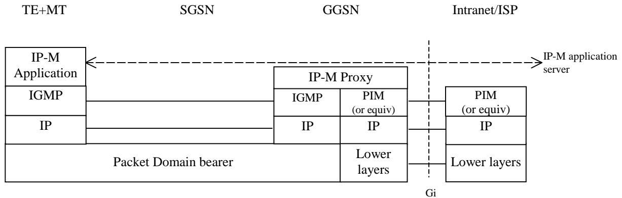
Figure 12: Protocol configuration for IP-Multicast handling (control plane)
