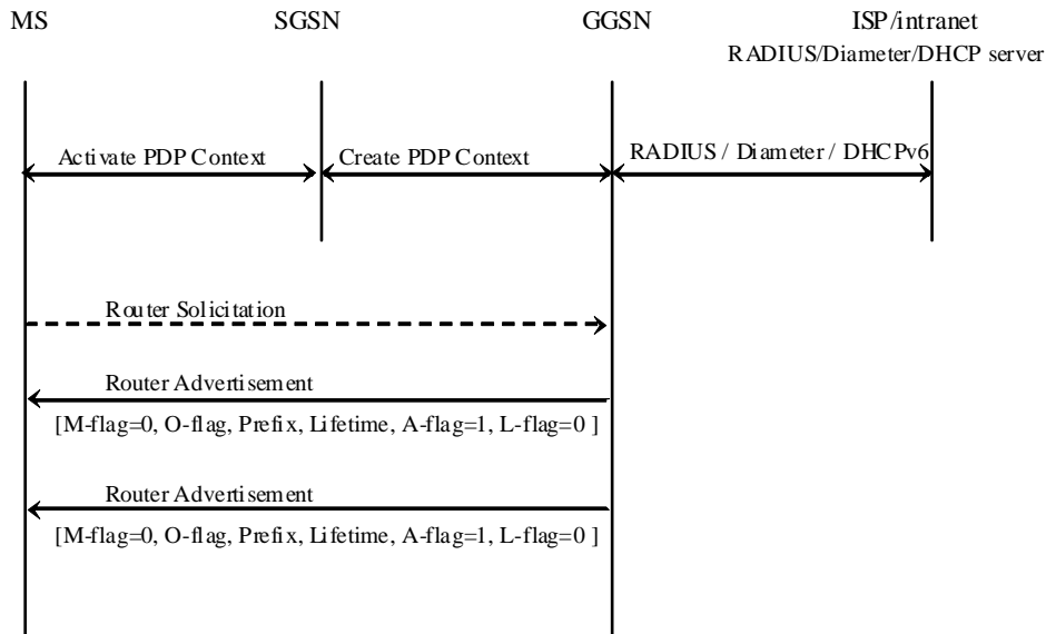
Figure 11bb: IPv6 Stateless Address Autoconfiguration
