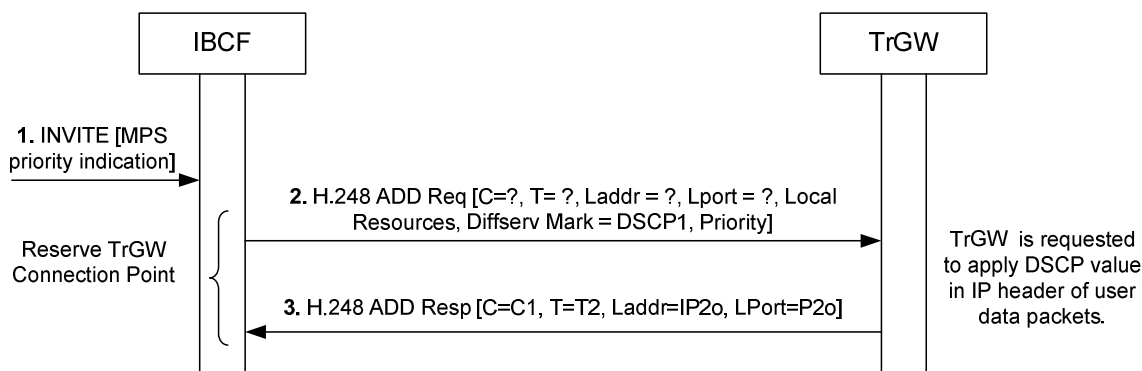
Figure 10.2.17.5.1: Request to reserve IMS resources and apply DSCP marking for MPS
