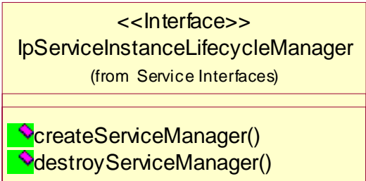
Figure: Service Instance Lifecycle Manager Package Overview
