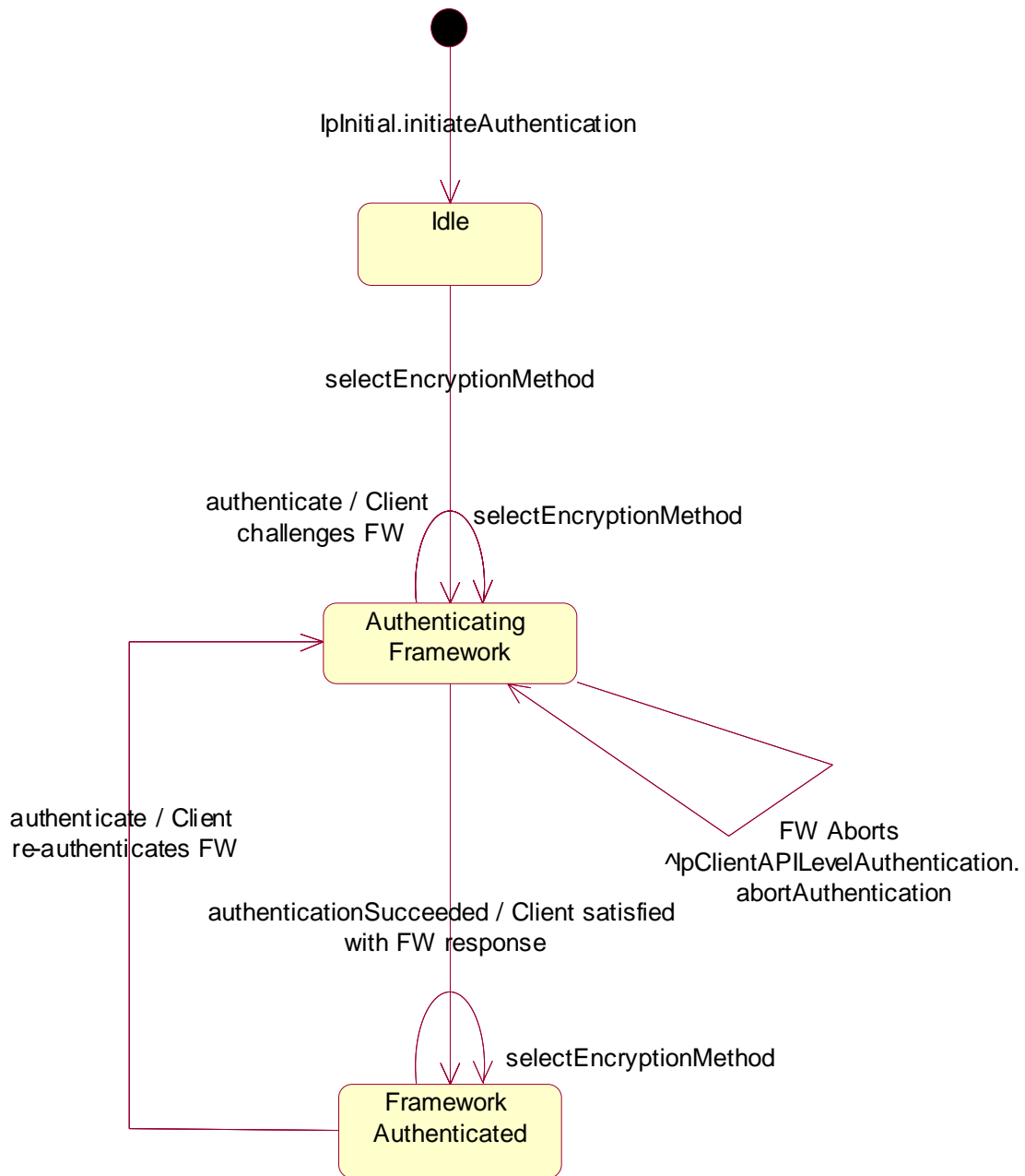
Figure : STD for IpAPILevelAuthentication: Client authenticates Framework using deprecated initiateAuthentication() and authenticate() method combination
