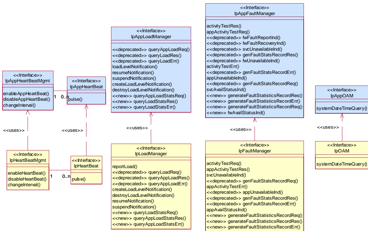
Figure: Integrity Management Package Overview
