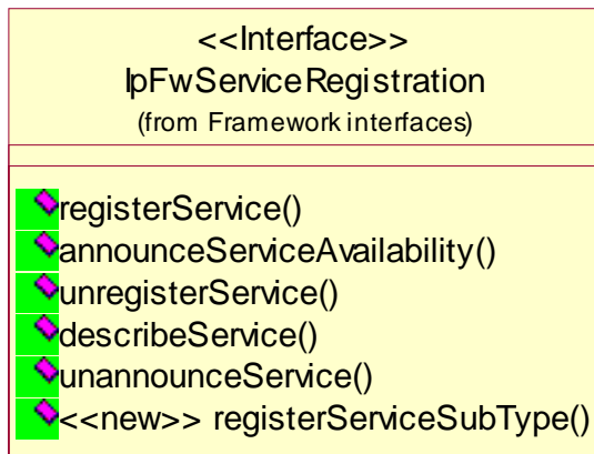
Figure: Service Registration Package Overview
