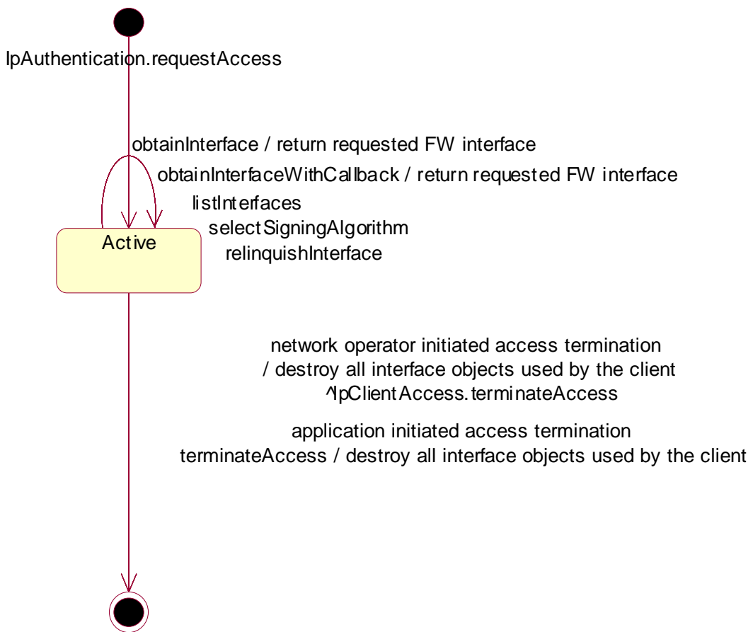
Figure : State Transition Diagram for IpAccess
