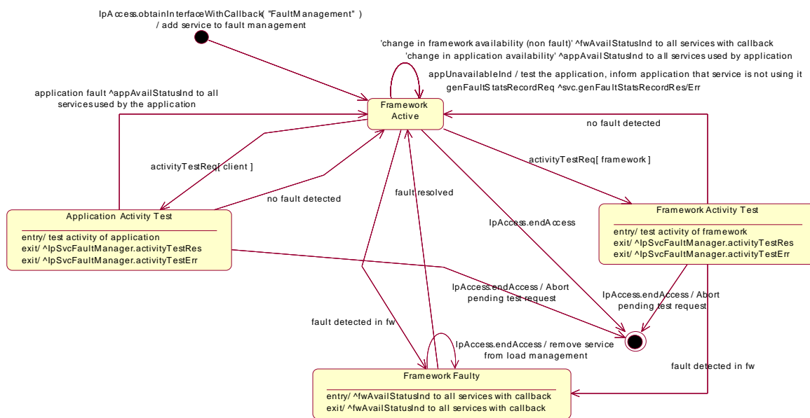
Figure : State Transition Diagram for IpFwFaultManager
