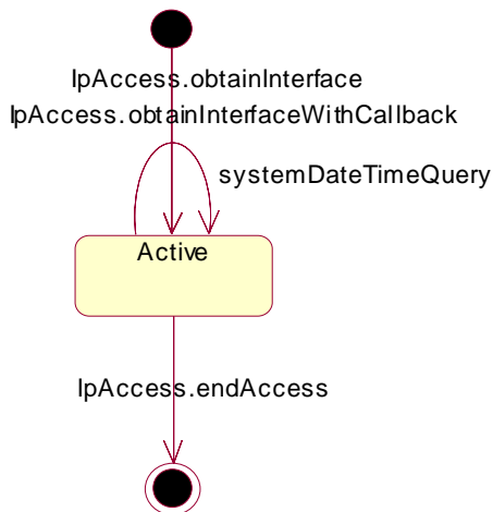
Figure : State Transition Diagram for IpOAM
