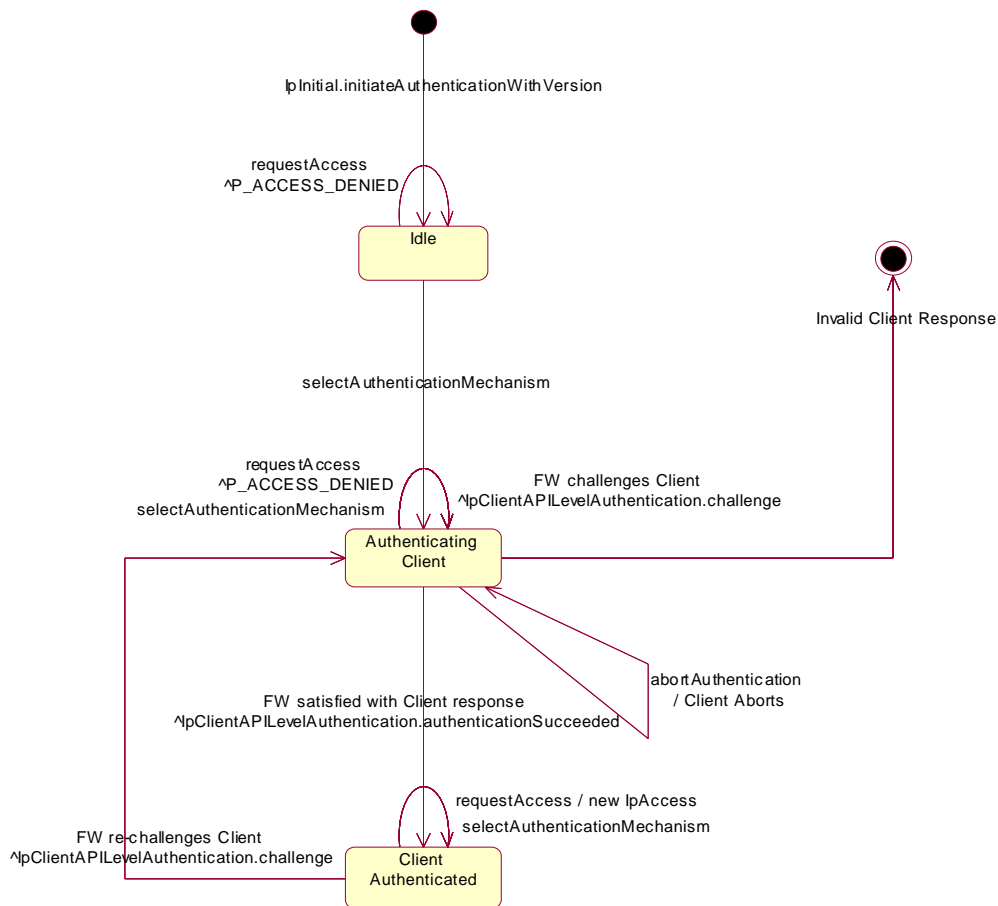
Figure : STD for IpAPILevelAuthentication: Framework authenticates Client using initiateAuthenticationWithVersion() and challenge() method combination
