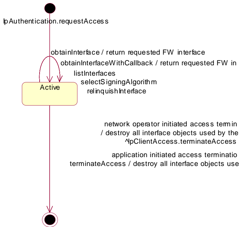
Figure : State Transition Diagram for IpAccess
