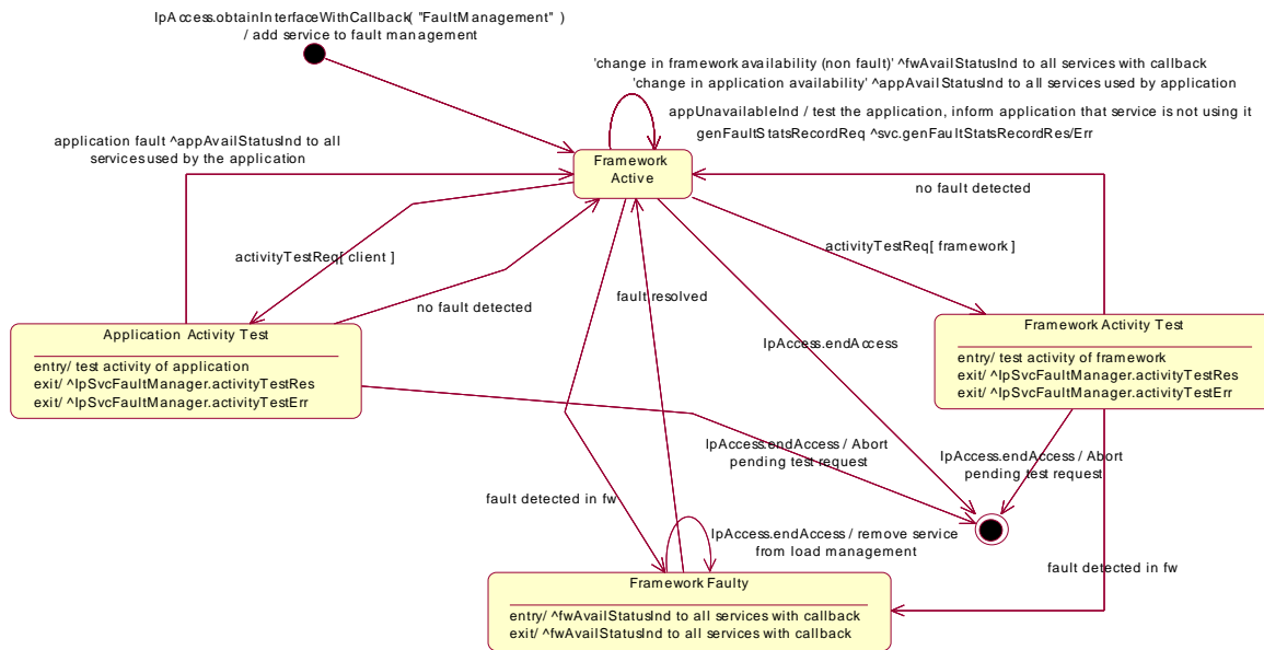
Figure : State Transition Diagram for IpFwFaultManager
