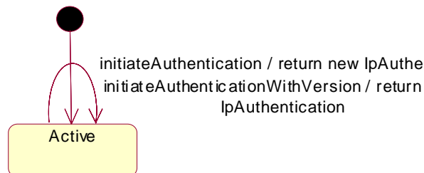
Figure : State Transition Diagram for IpInitial
