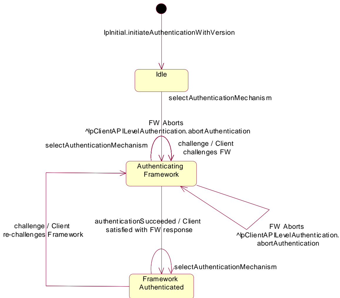
Figure : STD for IpAPILevelAuthentication: Client authenticates Framework using initiateAuthenticationWithVersion() and challenge() method combination
