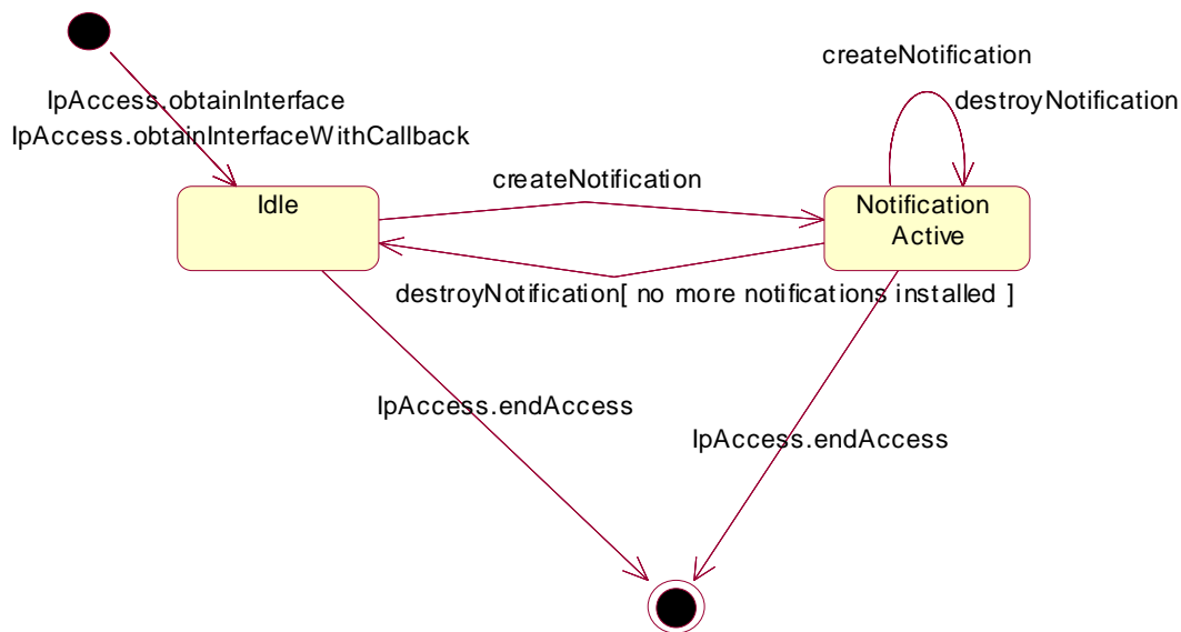
Figure : State Transition Diagram for IpEventNotification
