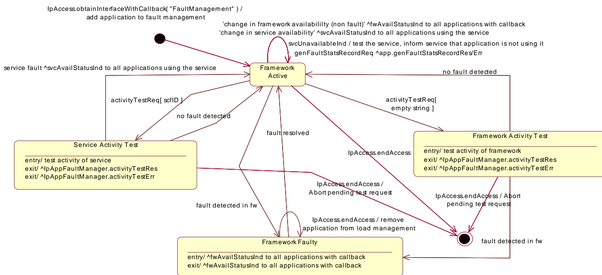
Figure : State Transition Diagram for IpFaultManager
