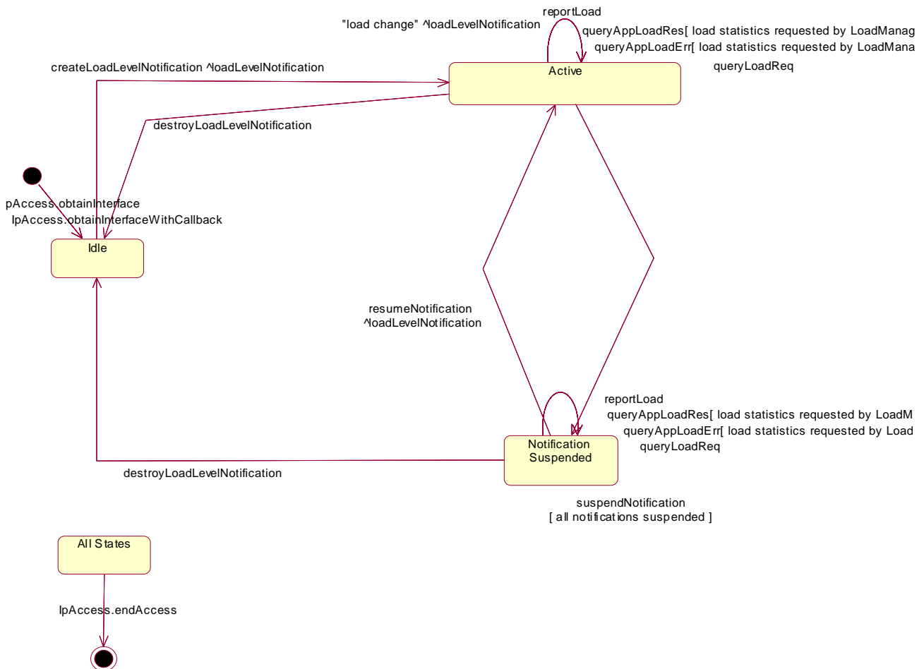
Figure : State Transition Diagram for IpFwLoadManager
