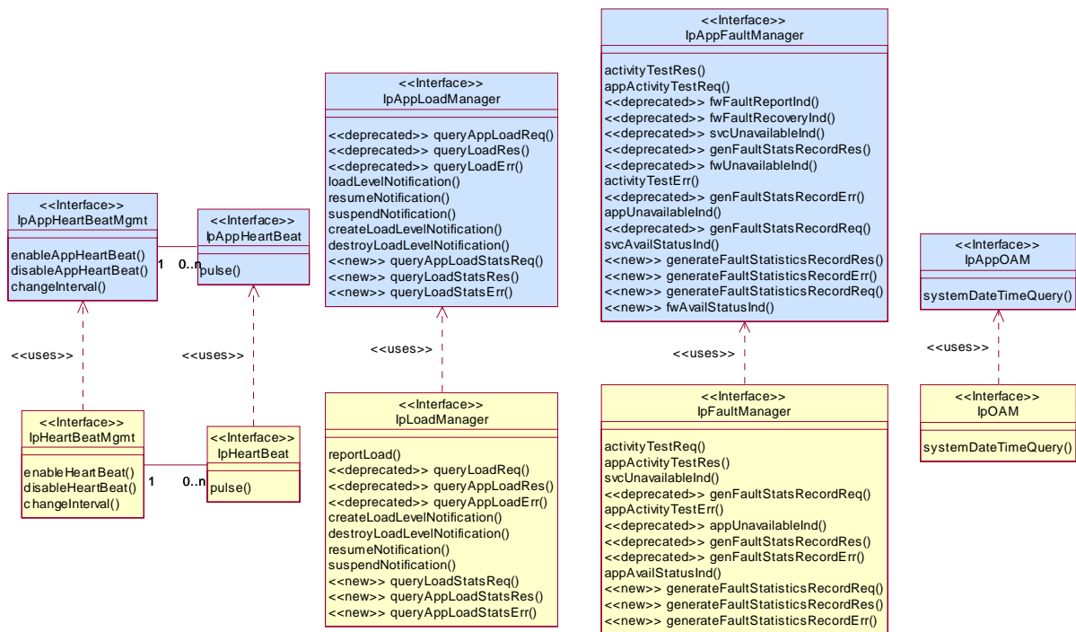
Figure: Integrity Management Package Overview
