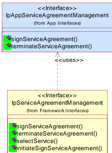
Figure: Service Agreement Management Package Overview
