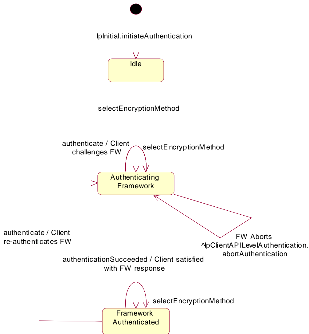
Figure : STD for IpAPILevelAuthentication: Client authenticates Framework using deprecated initiateAuthentication() and authenticate() method combination
