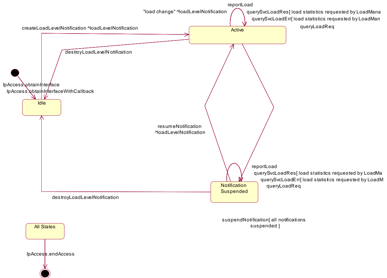
Figure : State Transition Diagram for IpLoadManager
