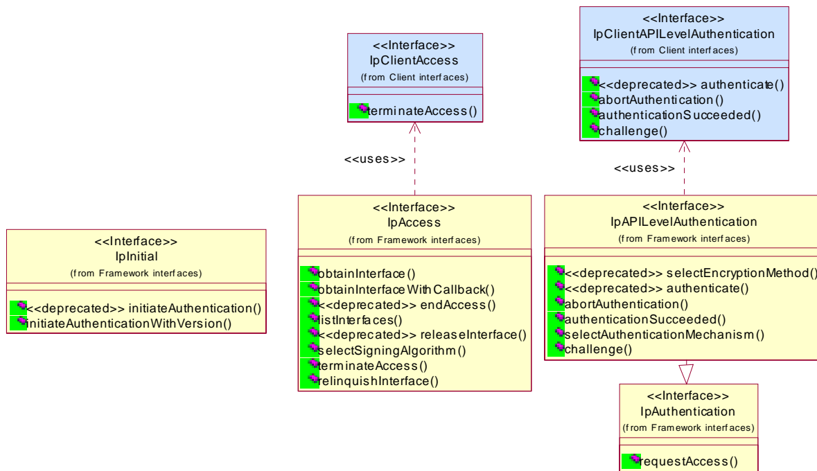
Figure: Trust and Security Management Package Overview
