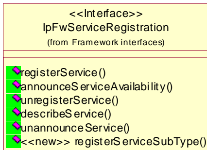
Figure: Service Registration Package Overview
