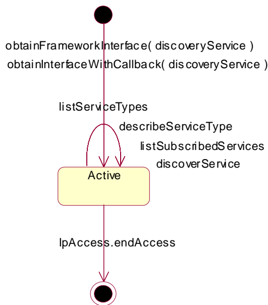
Figure : State Transition Diagram for IpServiceDiscovery
