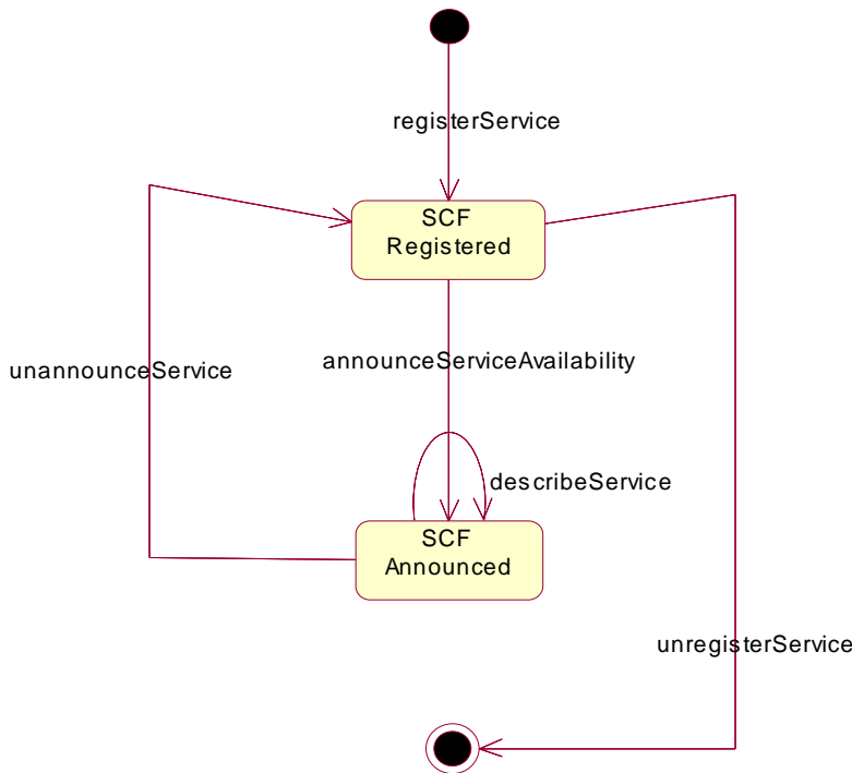
Figure : State Transition Diagram for IpFwServiceRegistration
