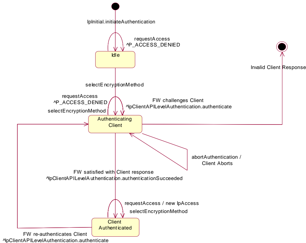
Figure : STD for IpAPILevelAuthentication: Framework authenticates Client using deprecated initiateAuthentication() and authenticate() method combination
