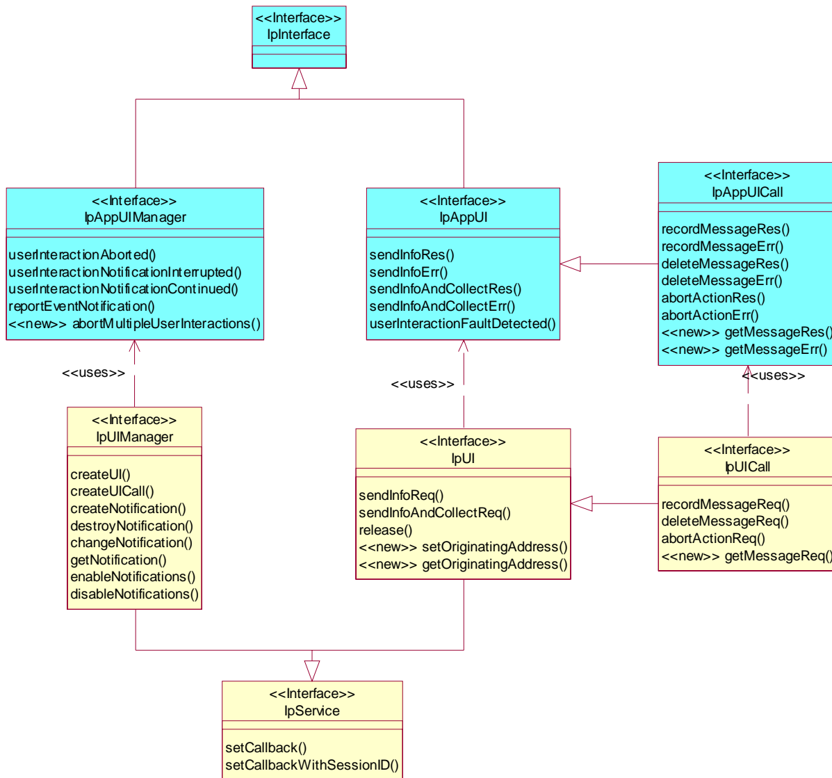
Figure: Generic User Interaction Package Overview
