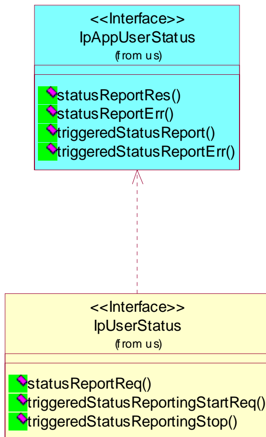
Figure: User Status Class Diagram
