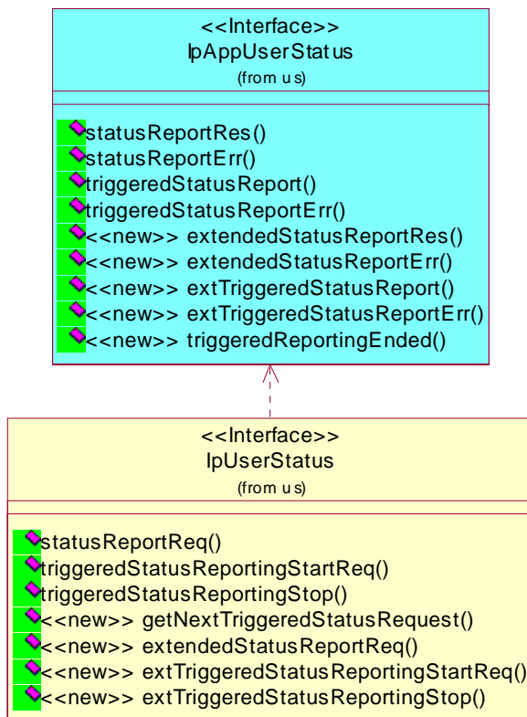
Figure: User Status Class Diagram
