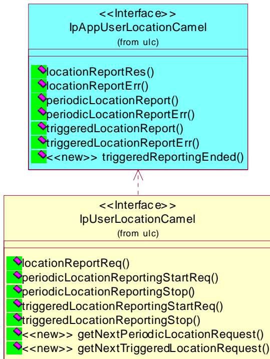
Figure: User Location Camel Class Diagram
