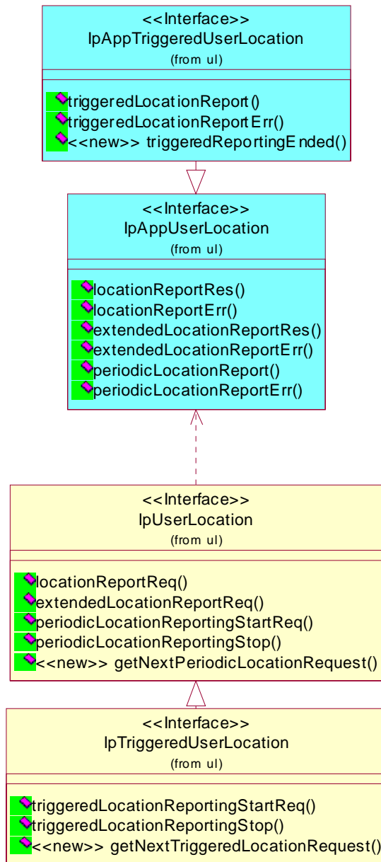
Figure: User Location Class Diagram
