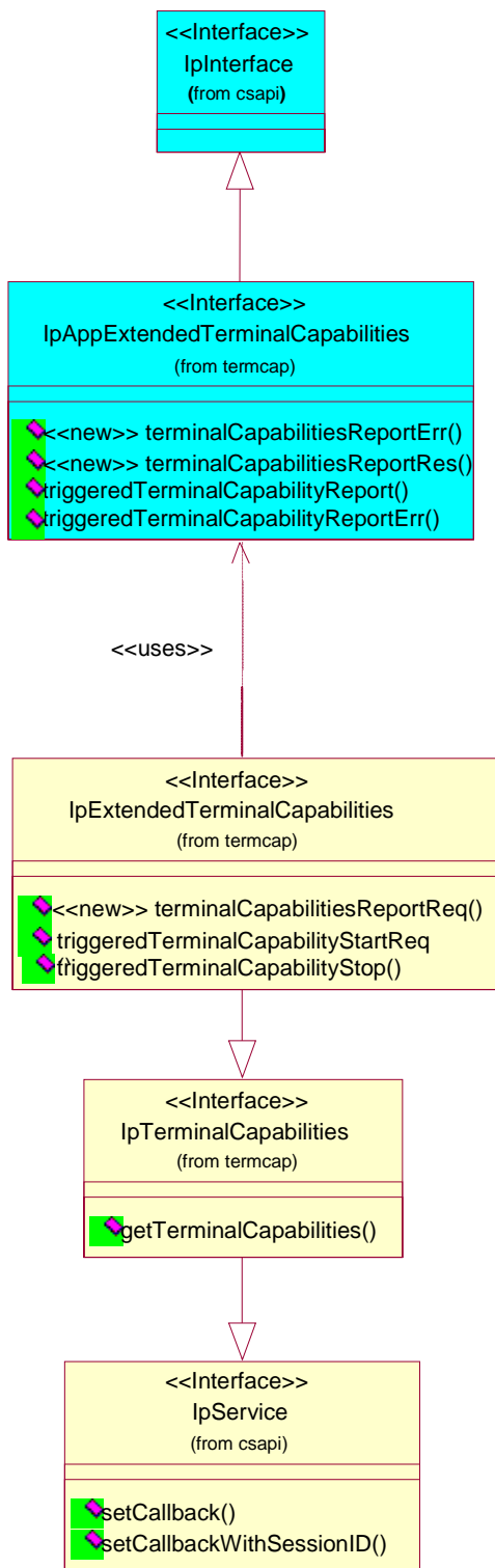
Figure: Terminal Capabilities Class Diagram
