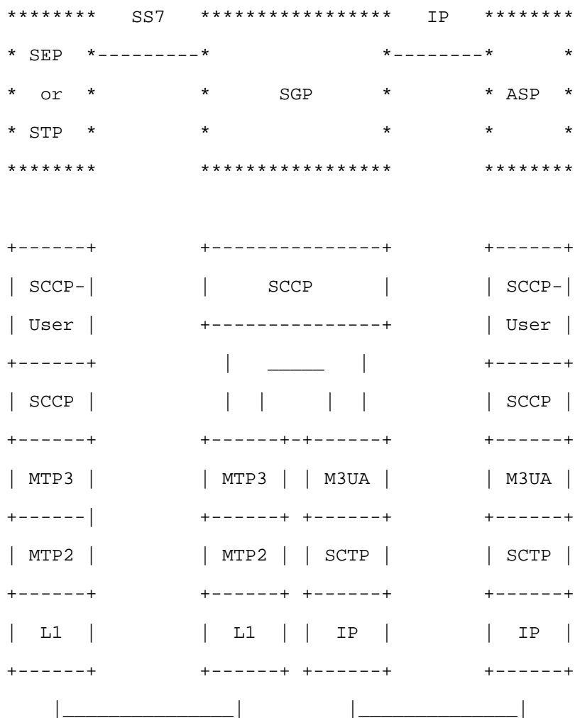
STP - SS7 Signalling Transfer Point
