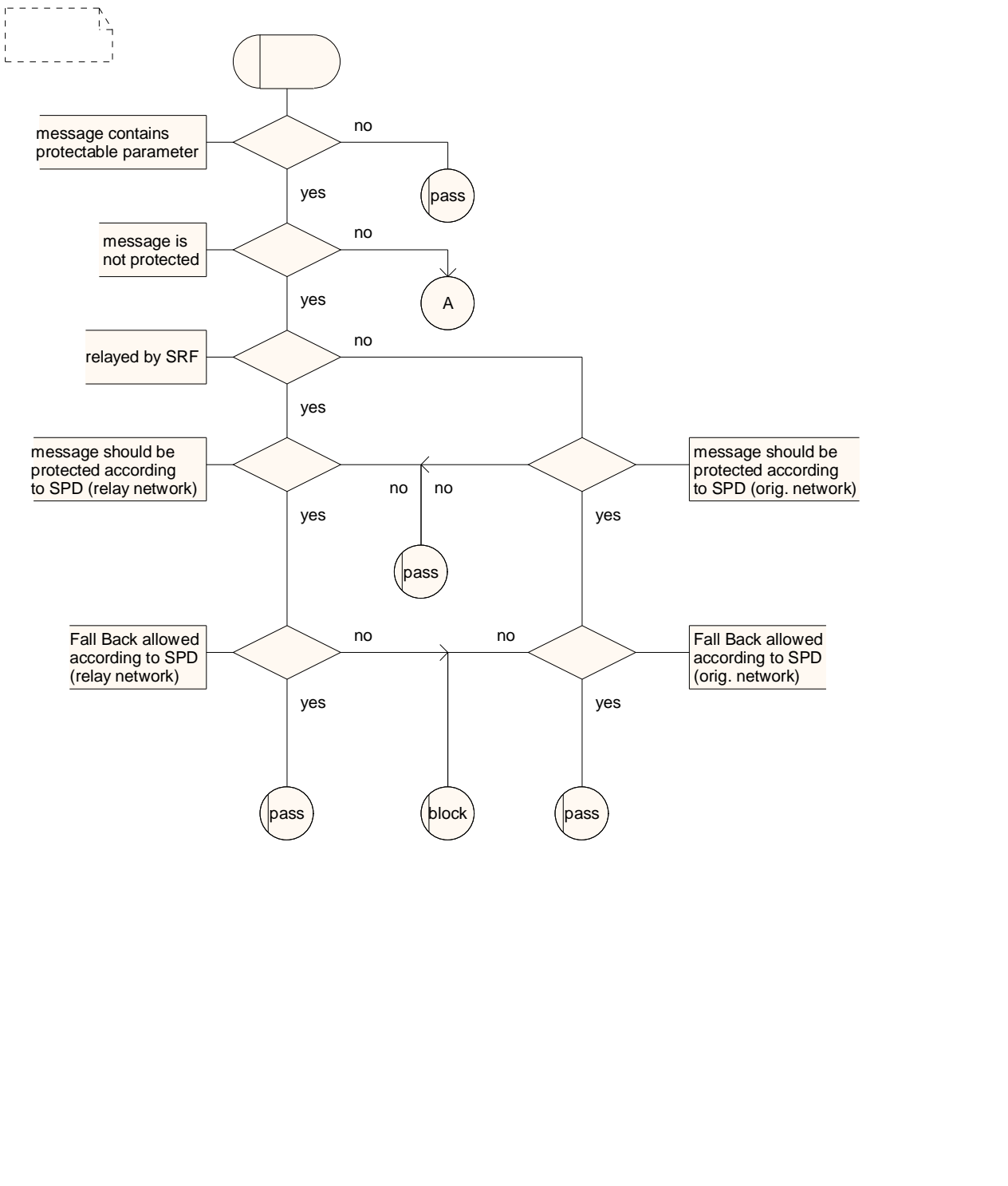
Figure 5.1.5 Macro Inbound_foreign_to_own (sheet 1 of 2)
