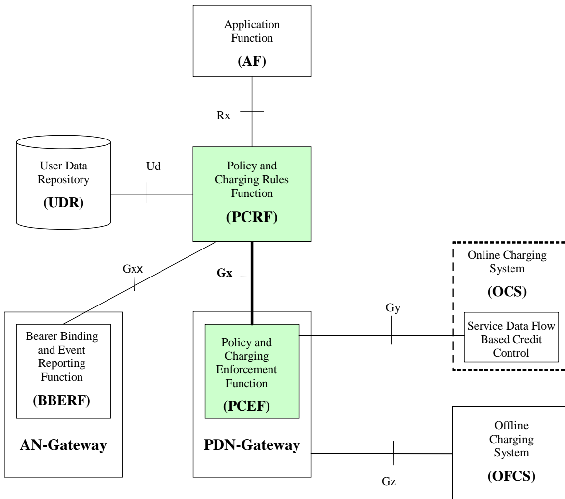
Figure 4.2: Gx reference point at the Policy and Charging Control (PCC) architecture with UDR
