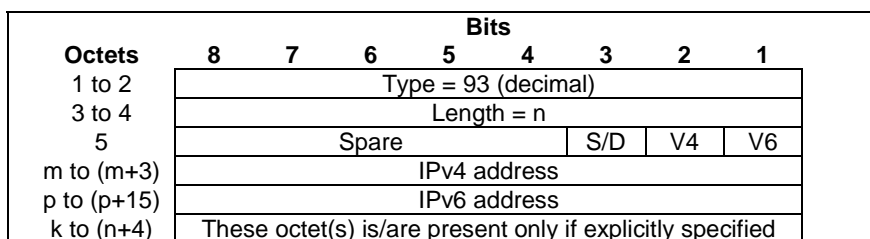
Figure 8.2.62-1: UE IP Address
